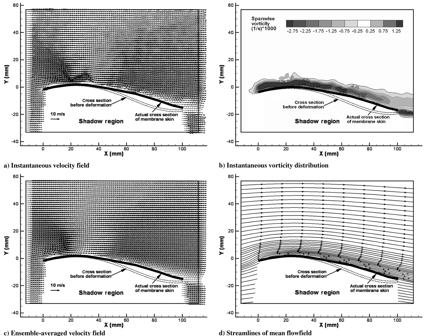
Fig. 8 PIV measurements in measurement plane 1 for the FM03 airfoil at AOA = 10.0 deg.
