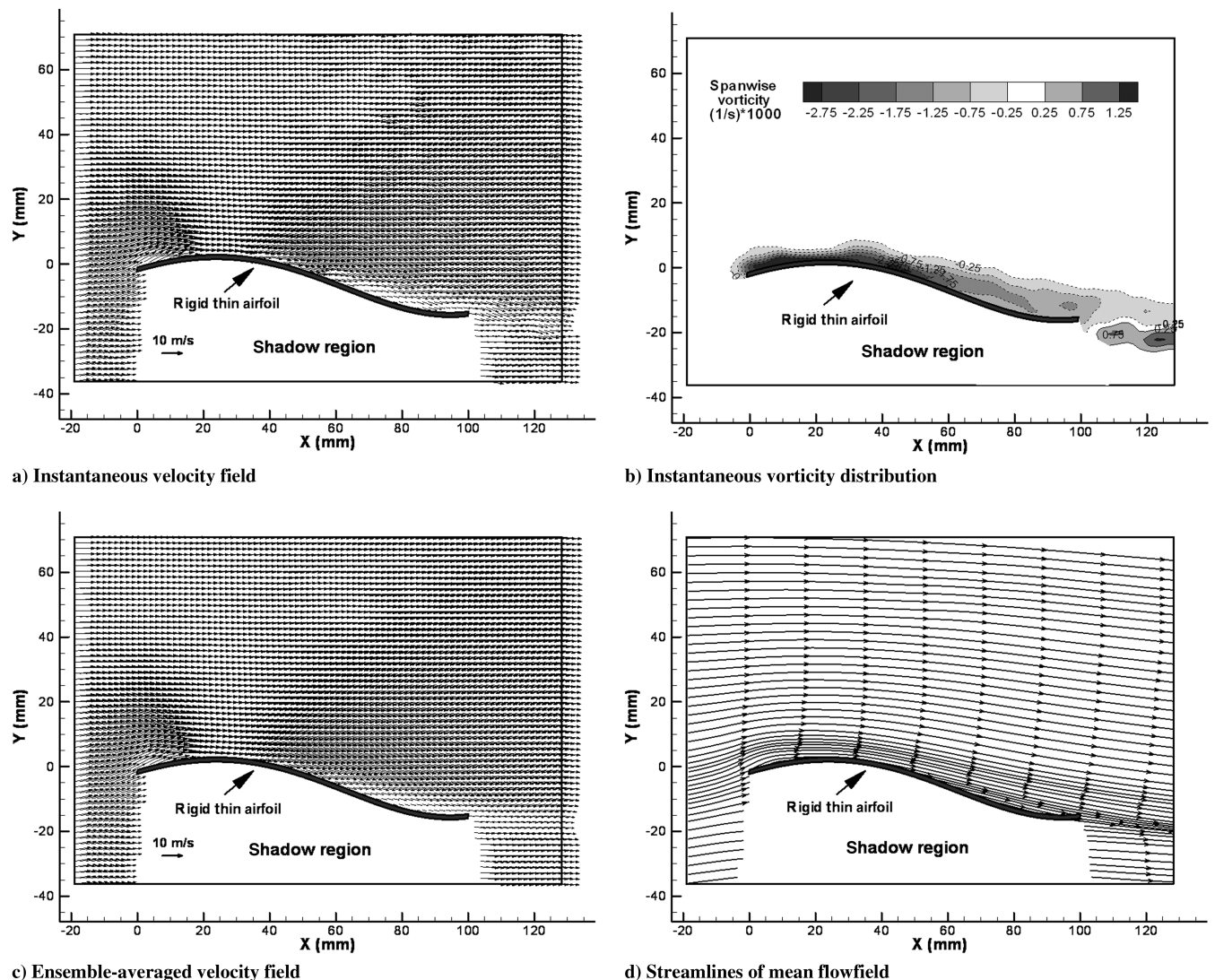
Fig. 5 PIV measurements in the midspan plane of the rigid thin airfoil at AOA = 6.0 deg.
