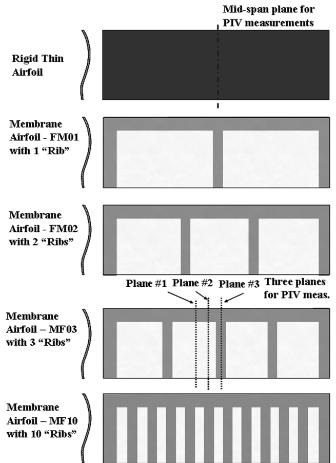
Fig. 2 Test airfoils and the locations of the cross planes for PIV measurements.
