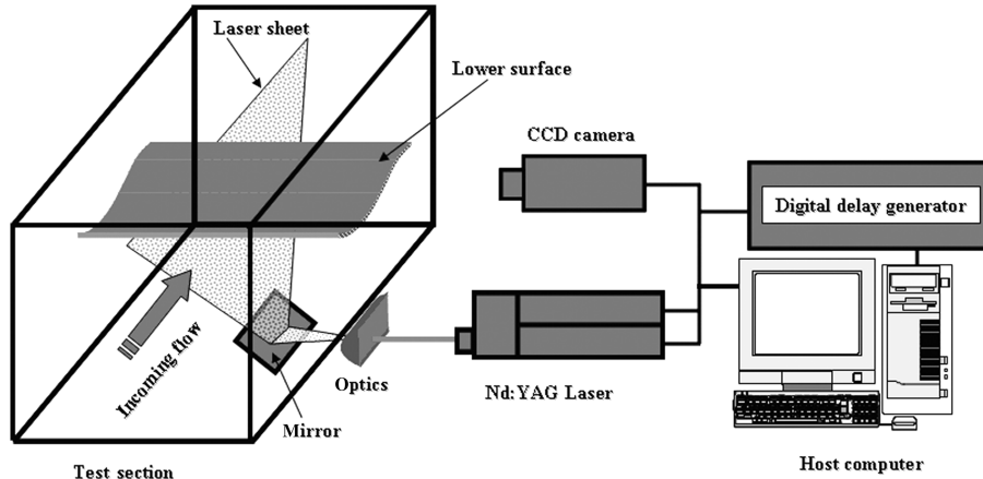
Fig. 3 Experimental setup.
