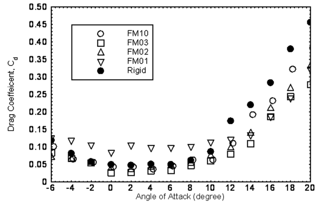
b) Drag coefficient vs angle of attack
