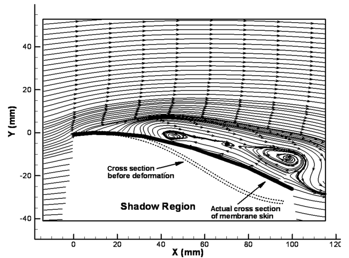
d) Streamlines of mean flowfield
