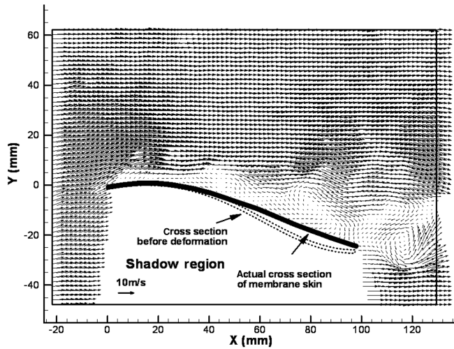
a) Instantaneous velocity field
