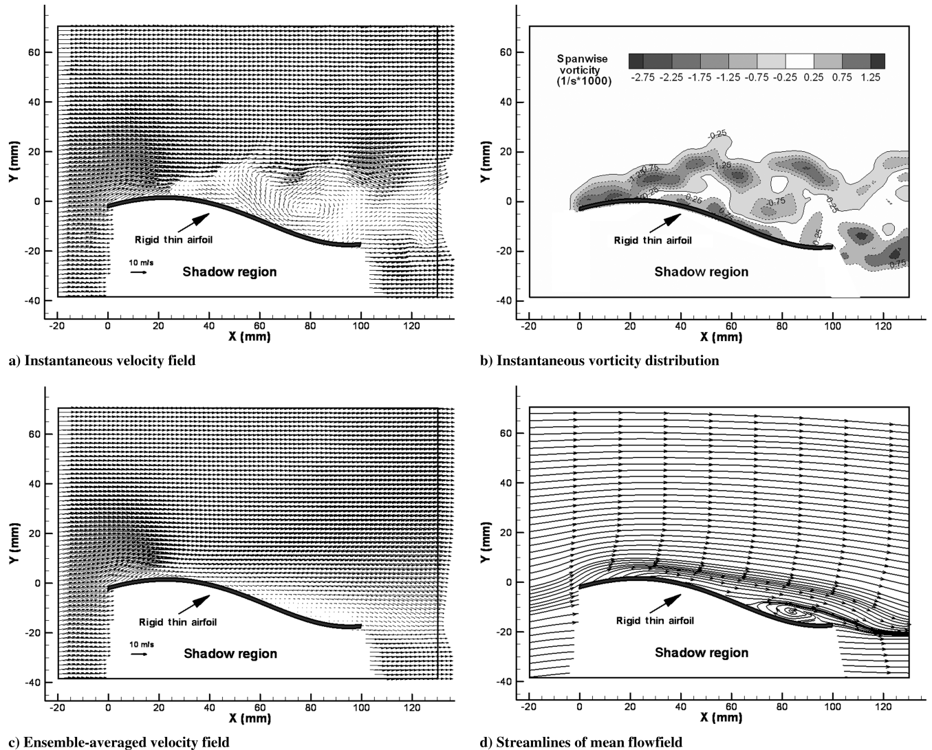
Fig. 6 PIV measurements in the midspan plane of the rigid thin airfoil at AOA = 10.0 deg.
