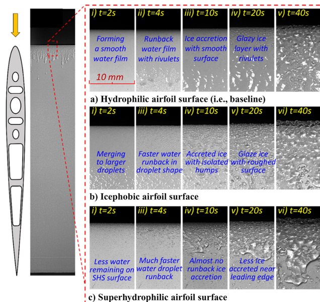
Fig. 4 Zoom-in view of the ice accretion process near the airfoil leading edge.
