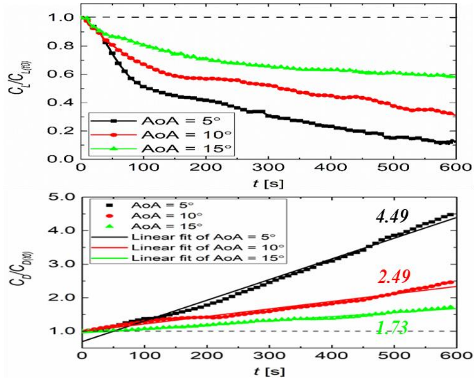
Fig. 5: Aerodynamic performance degradation of an ice accreting airfoil model (Gao et al, 2019).
