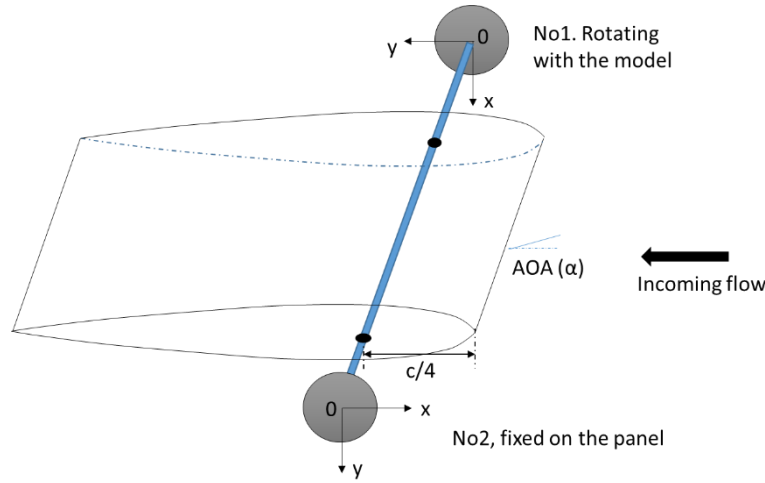
Figure 2: Configuration of the wing model in the wind tunnel relative to the force transducer. The force transducer origin is denoted by 0 .
