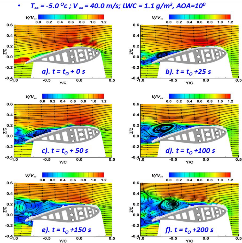
Fig. 3: PIV measurements to visualize the evolution of the airflow over the upper surface of an ice accreting airfoil model (Gao et al. 2019).
