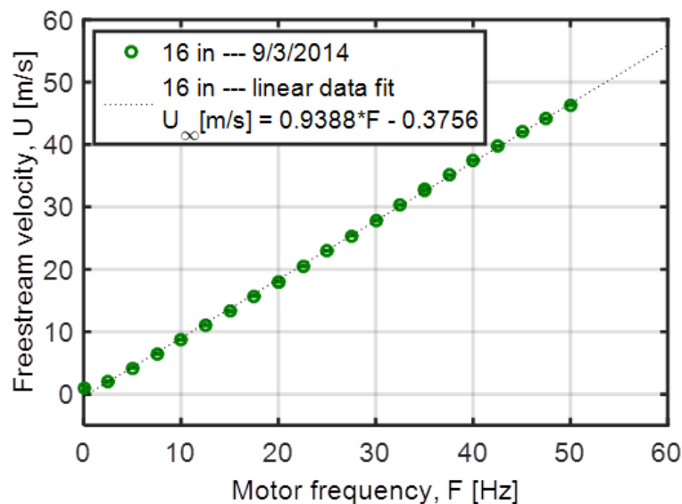
Figure 1. Wind tunnel airspeed versus motor frequency setting.
